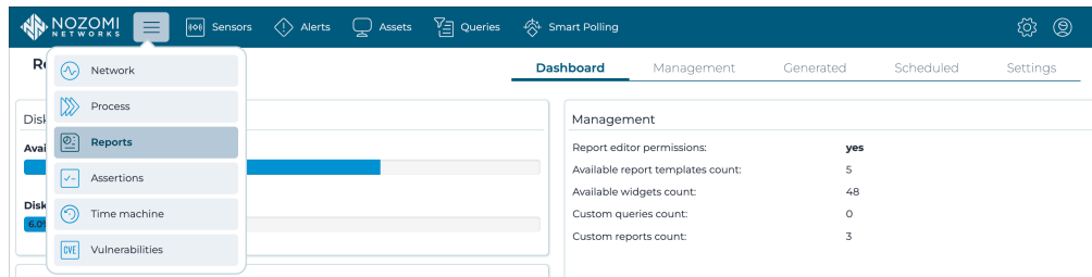
Figure 40. Reports page
