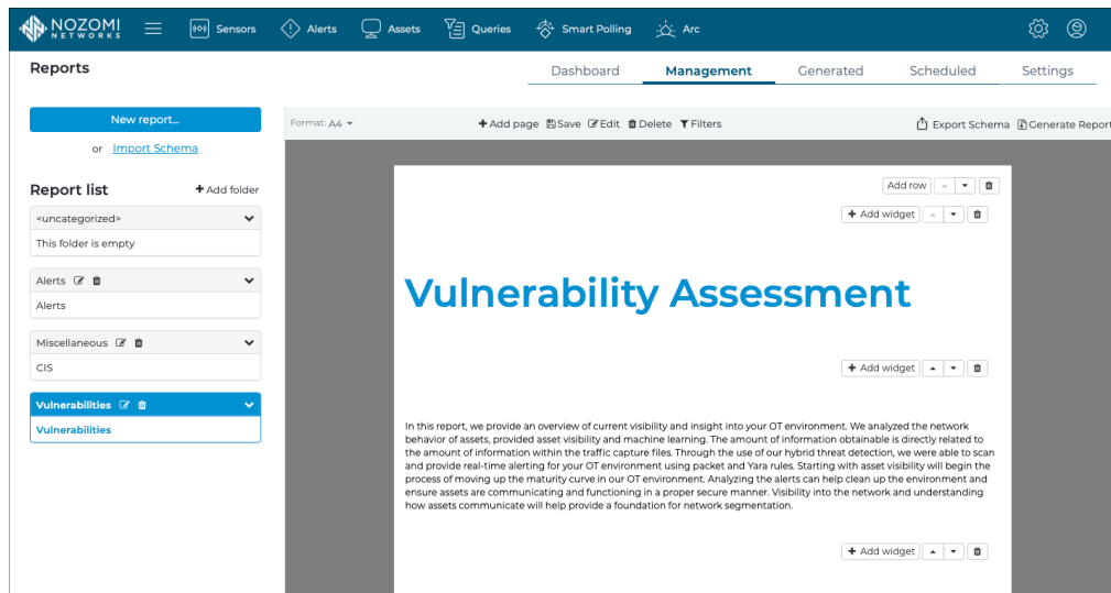
Figure 42. Management page
