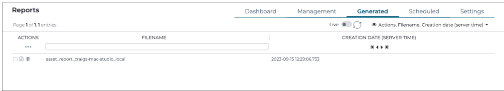
Figure 44. Generated page
