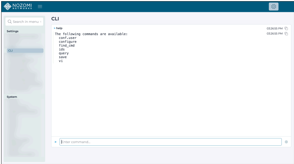
Figure 15. CLI page
