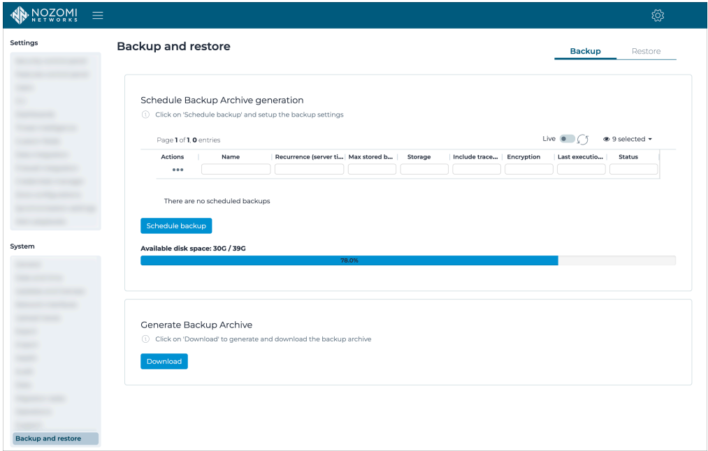
Figure 71. Backup page
