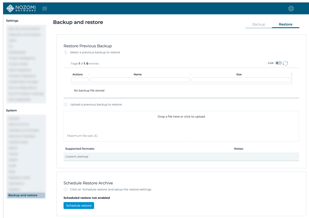
Figure 72. Restore page
