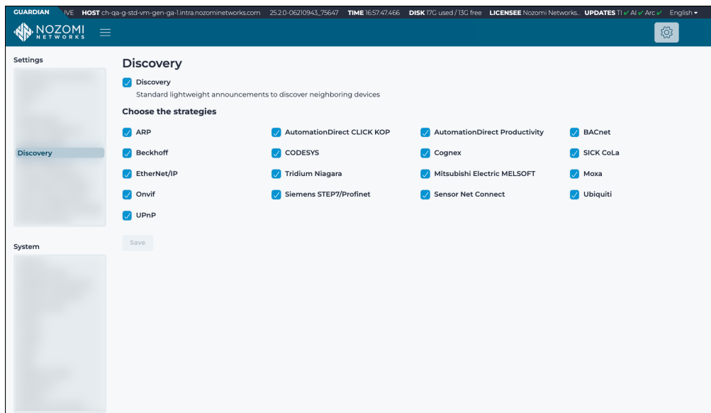
Figure 27. Discovery page
