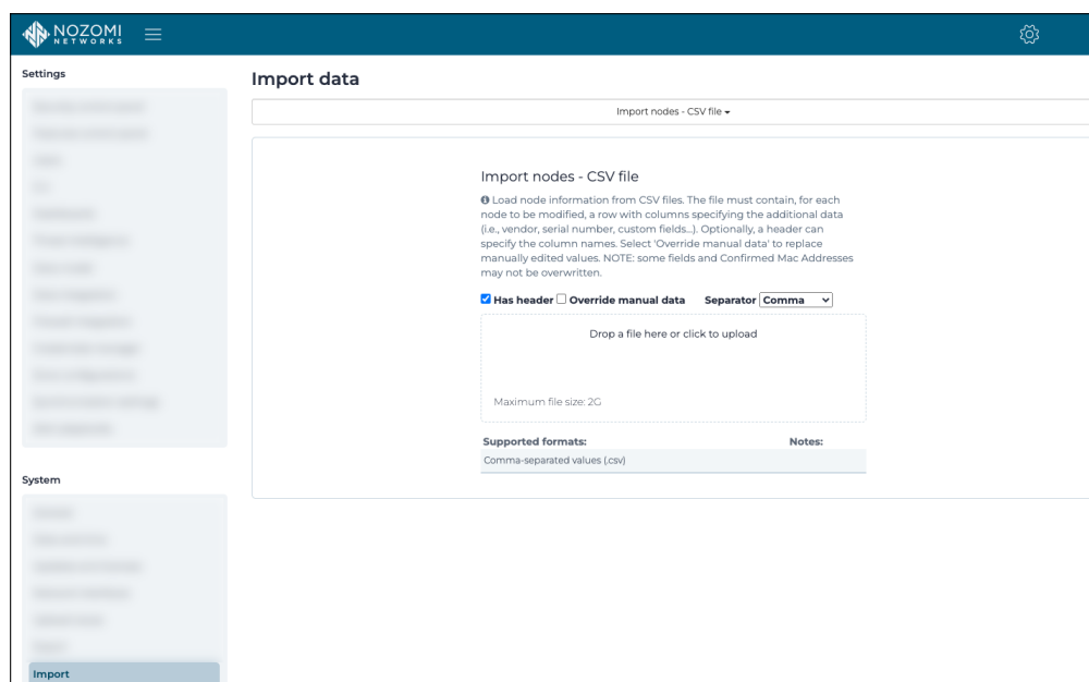
Figure 66. Import page
