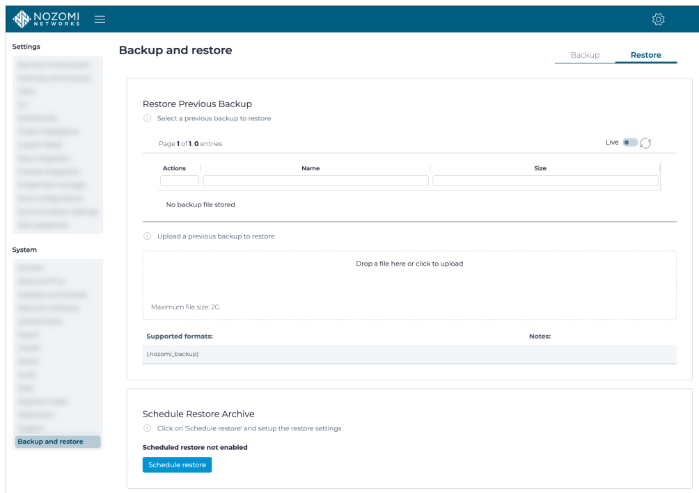
Figure 77. Restore page
