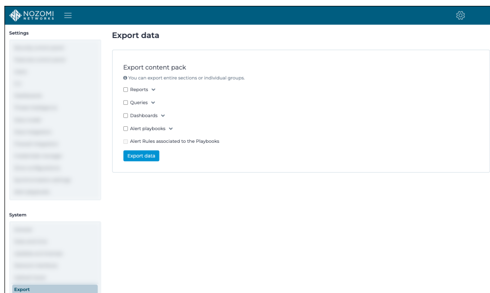
Figure 65. Export page
