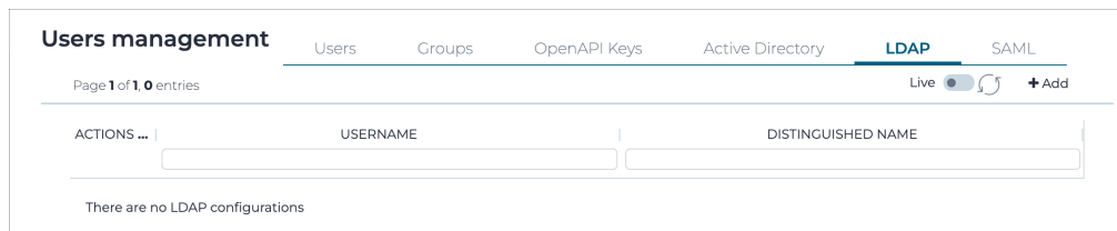
Figure 13. LDAP page
