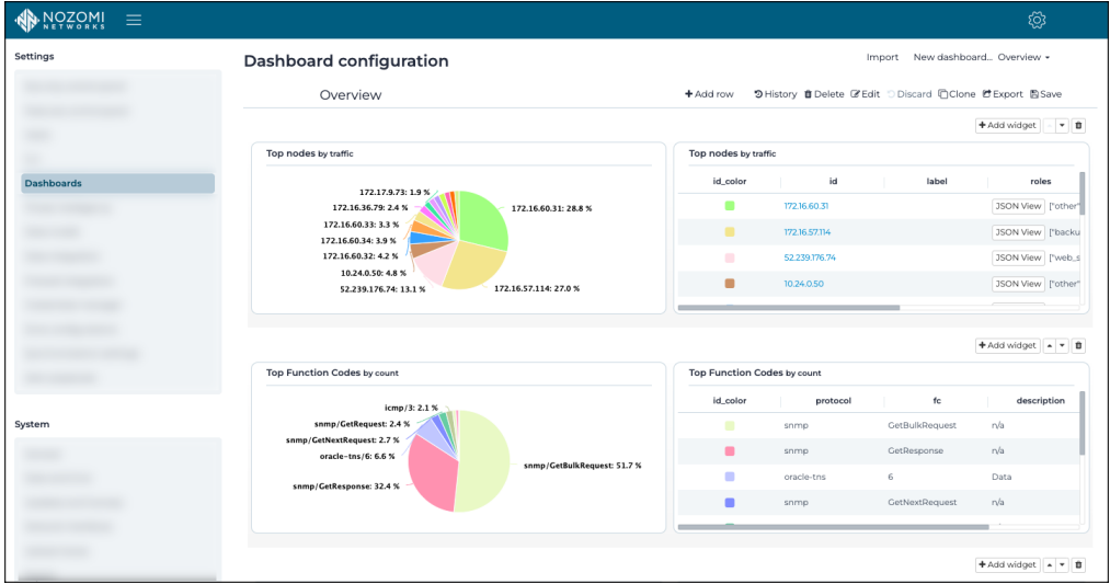
Figure 17. Dashboards page
