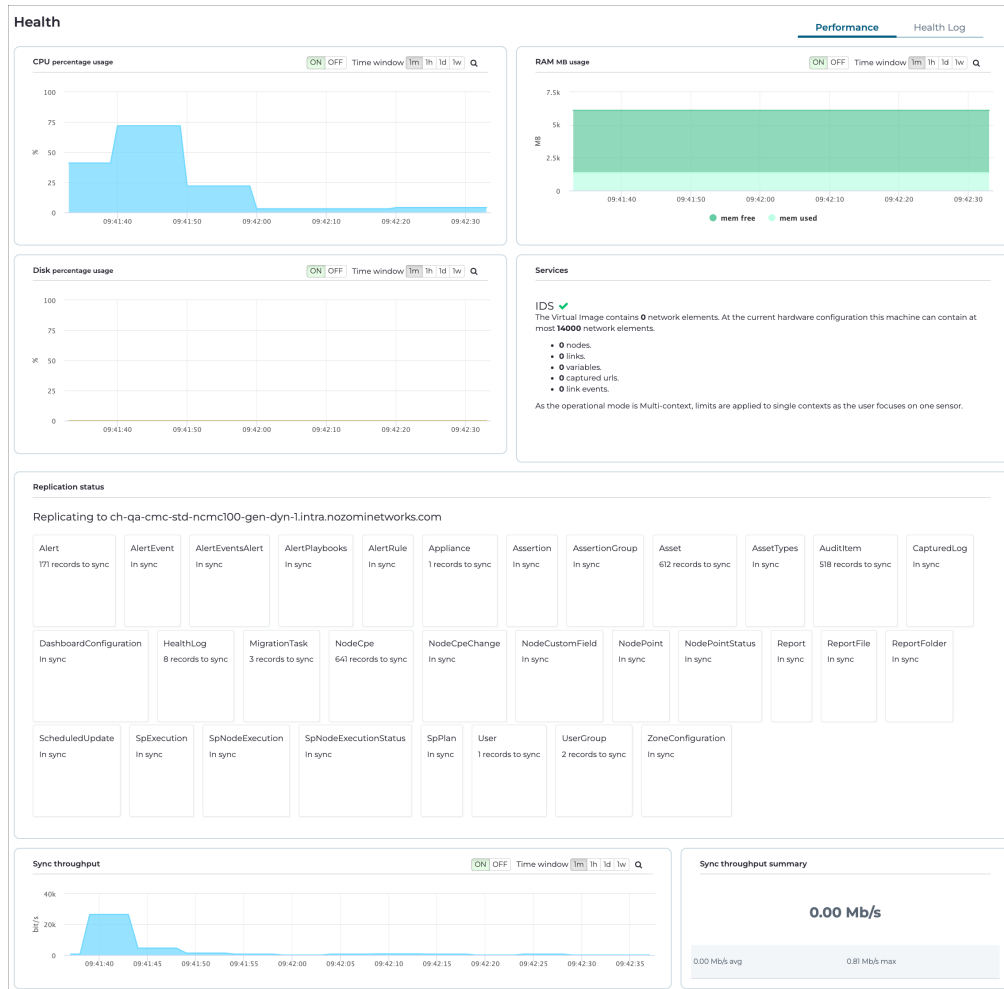
Figure 63. Performance page
