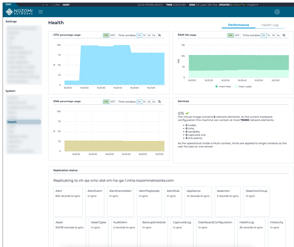
Figure 62. Health page
