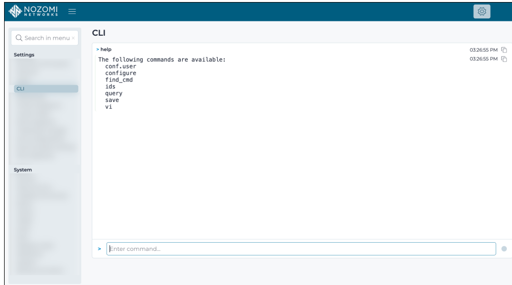
Figure 15. CLI page
