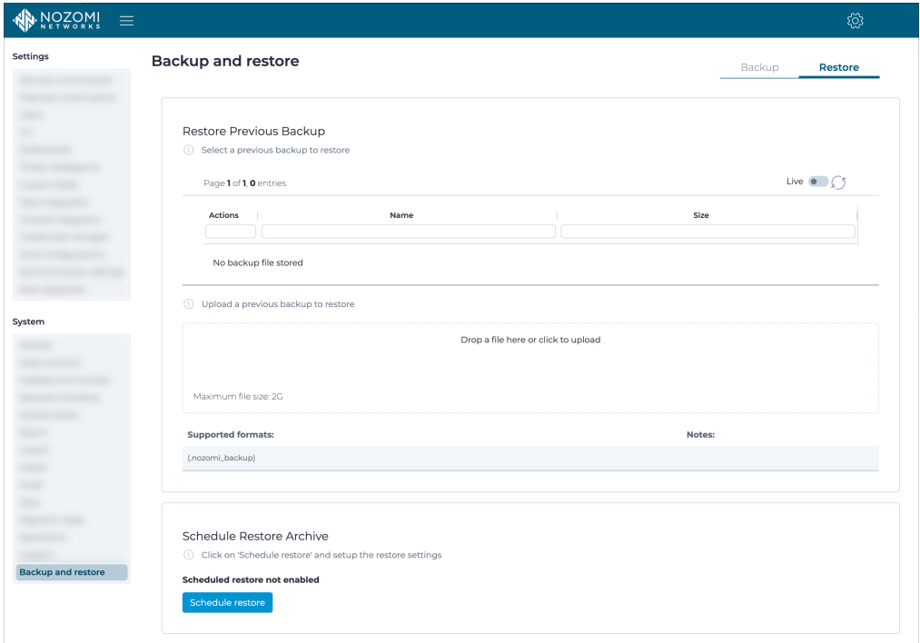
Figure 72. Restore page
