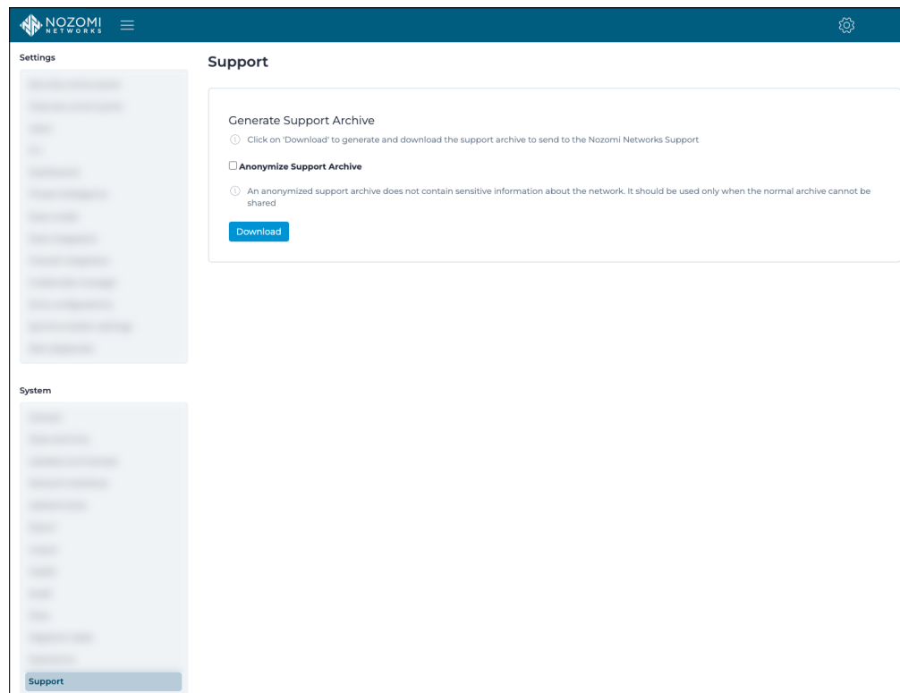
Figure 69. Support page
