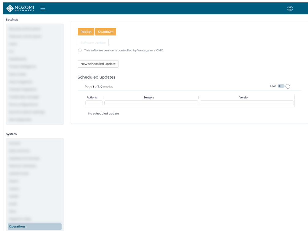
Figure 68. Operations page
