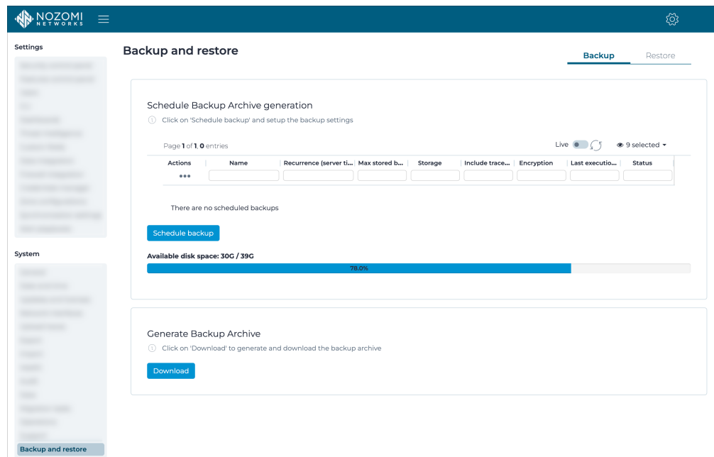
Figure 71. Backup page
